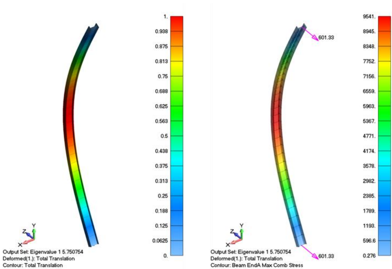
Figure 6: The first Eigenmode is shown deflected with a \lambda = 5.751 .
